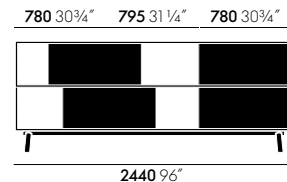
Kast, 2 HU (height unit), eight sliding doors
