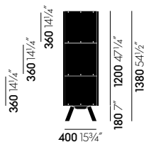
Kast, 3 HU (height unit), eight sliding doors
